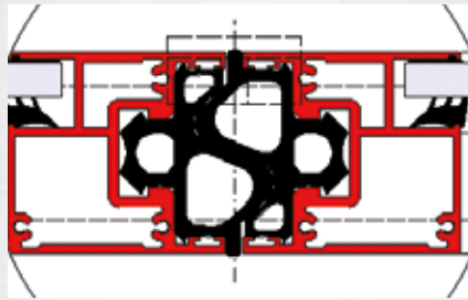
Central seal in the form of a labyrinth and made from hard material
